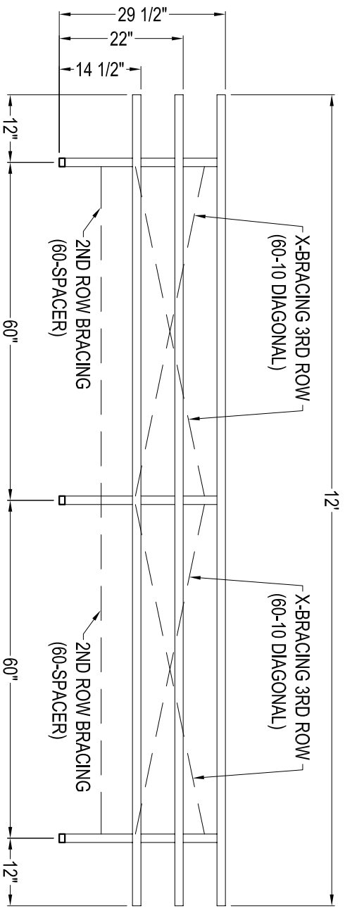
FRONT ELEVATION BL-3TR-12DR SCALE: 1/2" = 1'
