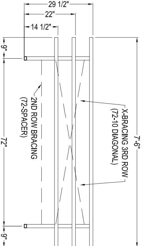
FRONT ELEVATION BL-3TR-7.5DR SCALE: 1/2" = 1'
