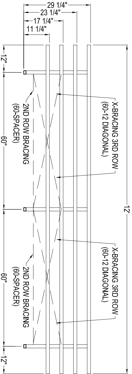
FRONT ELEVATION BL-4TR-12DR SCALE: 1/2" = 1'
